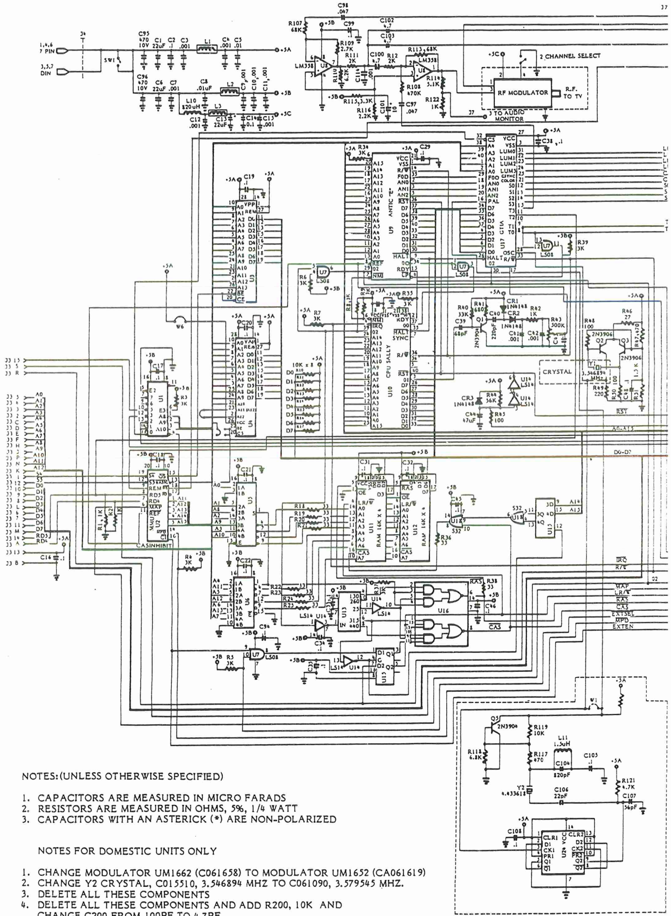
600XL SCHEMATIC
